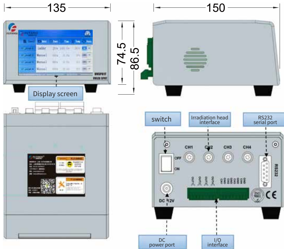
UVSP 81T (FOUR-CHANNEL UVLED POINT LIGHT SOURCE CONTROLLER)
