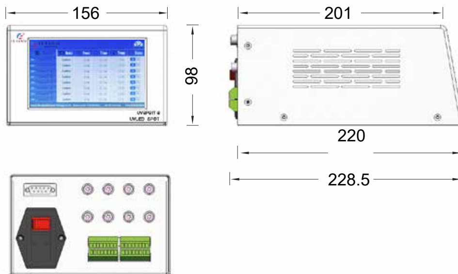
UVSP 81T-8 (8-CHANNEL UVLED POINT LIGHT SOURCE CONTROLLER)
